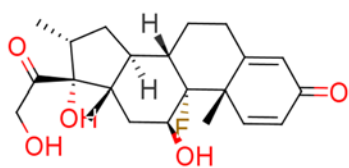
50-02-2
