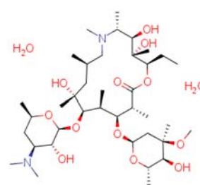
117772-70-0
