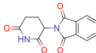
50-35-1
