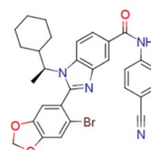
2100284-59-9
