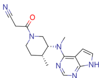
50-02-2
